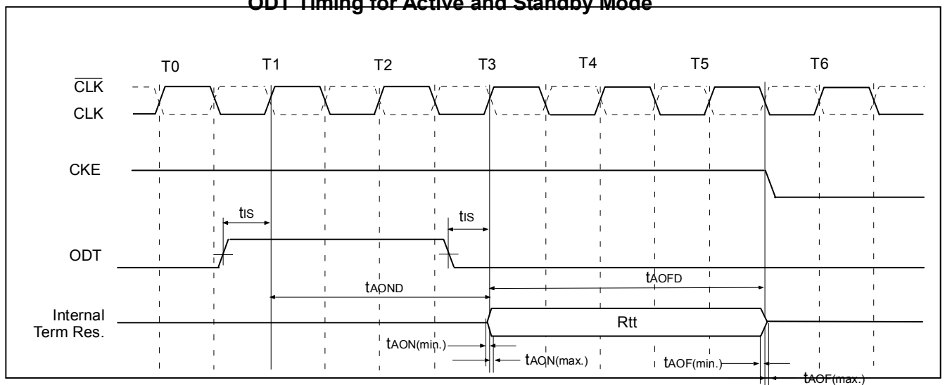
ODT Timing for Active and Standby Mode
